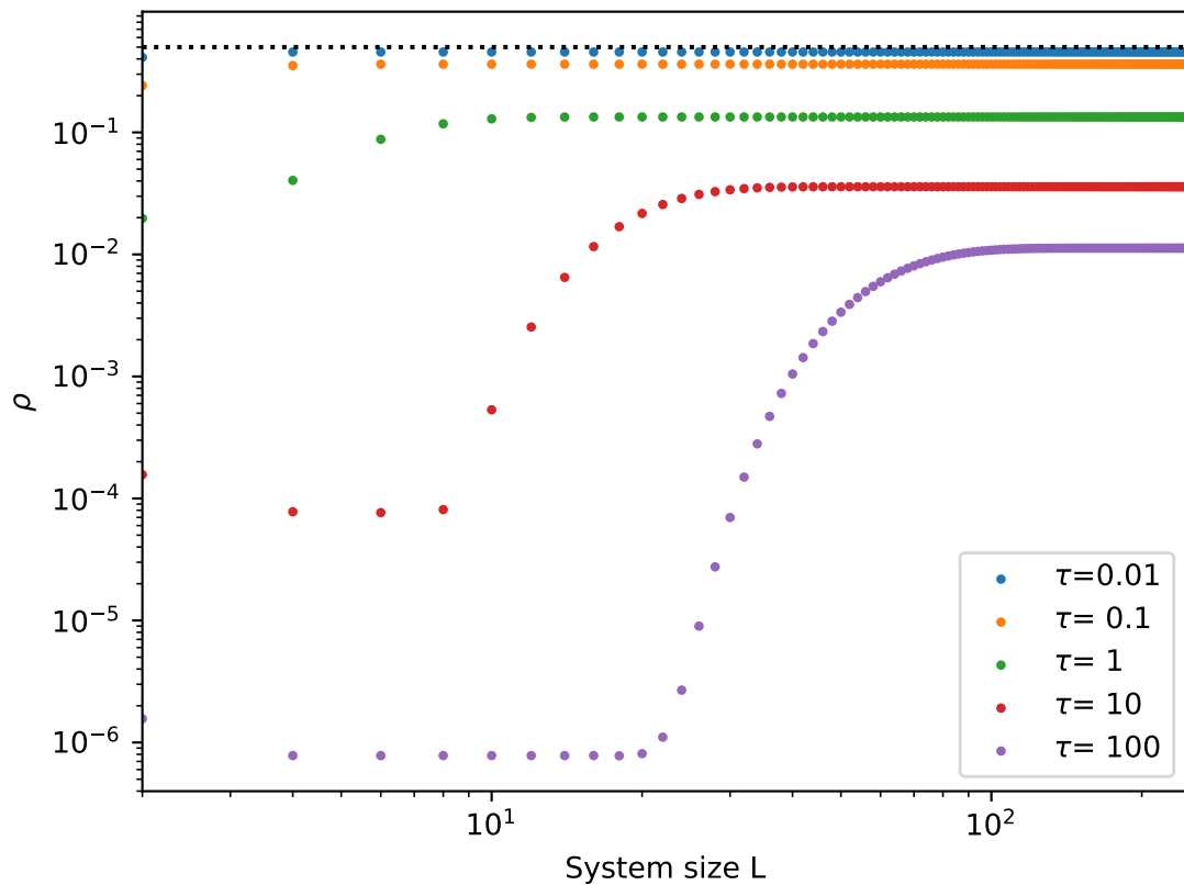
Defect density vs L at fixed \tau
